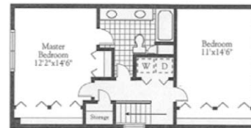
Upper Level Plan
