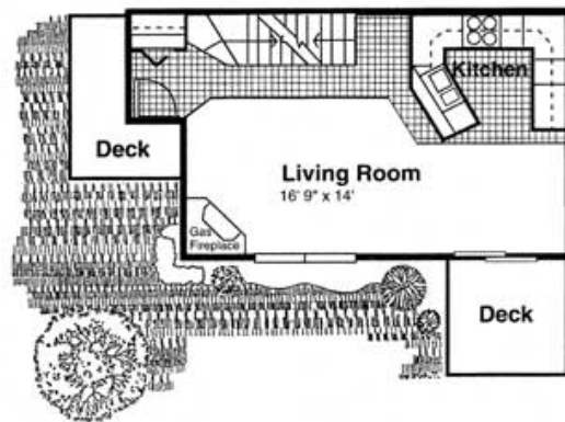
MAIN FLOOR
